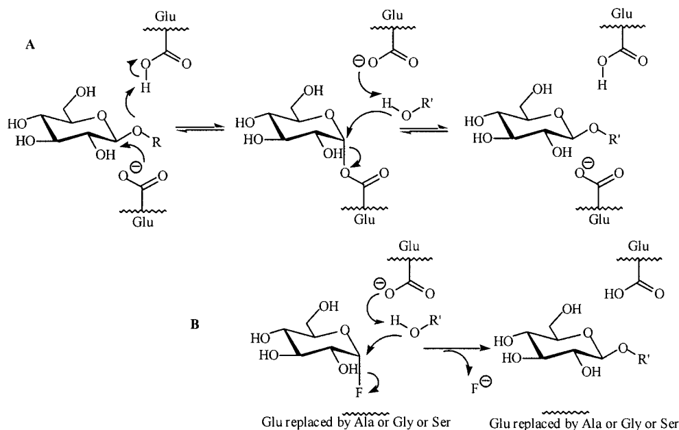
Scheme 1. Transglycosidation mechanism: A) with retaining glycosidases, and B) with glycosynthases.
