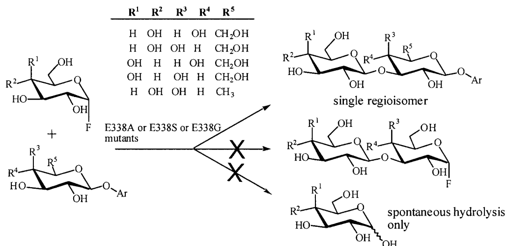
Scheme 2. Reactions catalyzed by Tt - \beta -Gly glycosynthase mutants.
