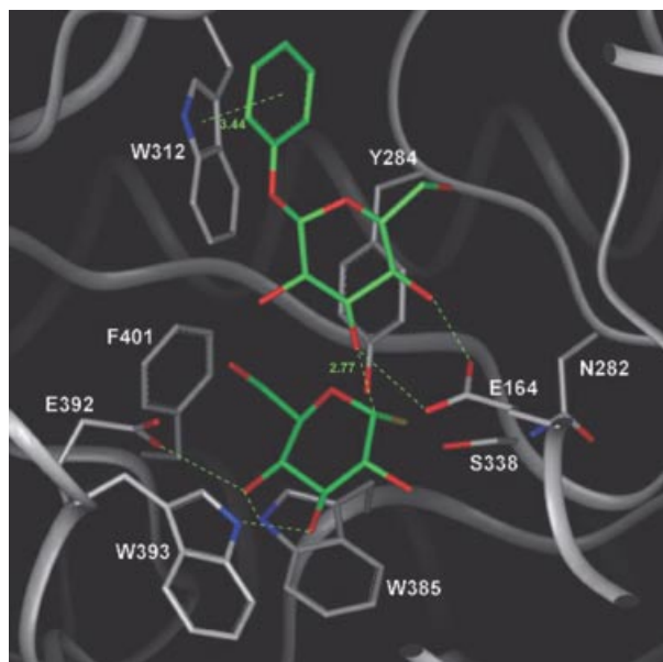
Figure 2. Molecular modeling, in the active site, of the disposition of reactants before the transglycosidation reaction catalyzed by E338S glycosynthase, with \alpha -GlcF as donor and \beta -GlcPh as acceptor. An energy minimum was obtained when stacking occurred between the phenyl group of \beta -GlcPh and tryptophan 312. Moreover, the relative dispositions of the reactants, stabilized by several hydrogen bonds, were in agreement with the formation of a \beta -(1 \rightarrow 3) glycosidic bond.
