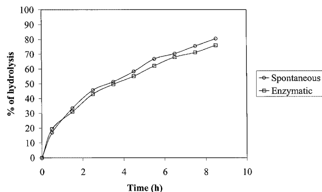
Figure 1. Comparison between spontaneous and enzymatically catalyzed hydrolysis of \alpha -glucosyl fluoride {experimental conditions: E338G glycosynthase, T = 55\text{ }^{\circ}\text{C} , \text{pH} = 7.8 , [\alpha\text{-GlcF}] = 50\text{ mmol L}^{-1} }.
